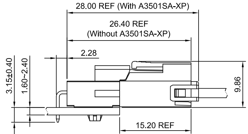
Mated with A3501WRE-F-XP
